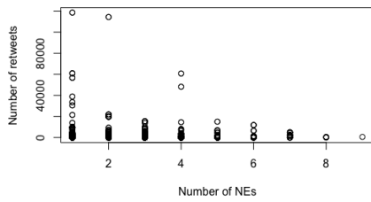
(e) Retweets vs NEs in Trump
