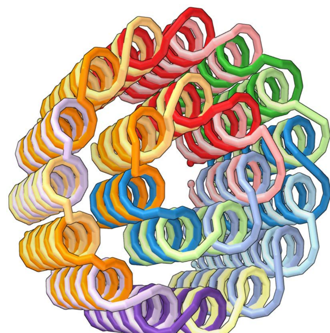
nanotubes
