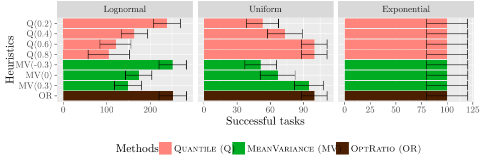
Figure 2: Number of successfully executed tasks for each heuristic with three distributions (Lognormal, Uniform, Exponential) of same expected value \mu = 1 and standard deviation \sigma = 3 , with a budget and deadline b = d = 100 (which means that a single machine is enrolled). Each heuristic is run 100,000 times for each scenario. The error bars are computed with the mean plus/minus two standard deviations of the number of successes. The lognormal distribution has parameters \alpha \approx -1.15 and \beta \approx 1.52 to have an expected value \mu = 1 and a standard deviation \sigma = 3 , and the optimal cutting threshold for OPTRATIO is l \approx 0.1 ). The exponential distribution has shape \lambda = 1 and the cutting threshold is arbitrarily set to l = 2 . The uniform distribution has parameters a = 0 and b = 2 , and the cutting threshold is l = 2 .
