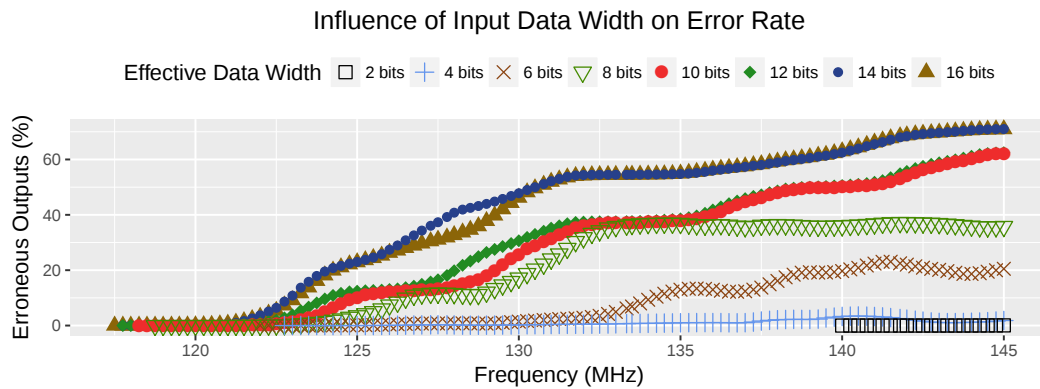
Figure 5: Percentage of corrupted outputs as a function of operating frequency over 400 images. Effective Data Width of n means 16 - n most significant bits were set to zero. Data points with zero observed error are not plotted - the bottom points have small but non-zero error rate.
