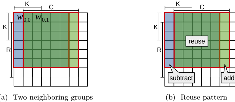
Figure 3: The reuse between two input groups corresponding to weights w_{0,0} and w_{0,1} . The sum of all elements in group w_{0,1} can be computed by addition/subtraction of columns from that of w_{0,0} , instead of repeating R \times C additions.
