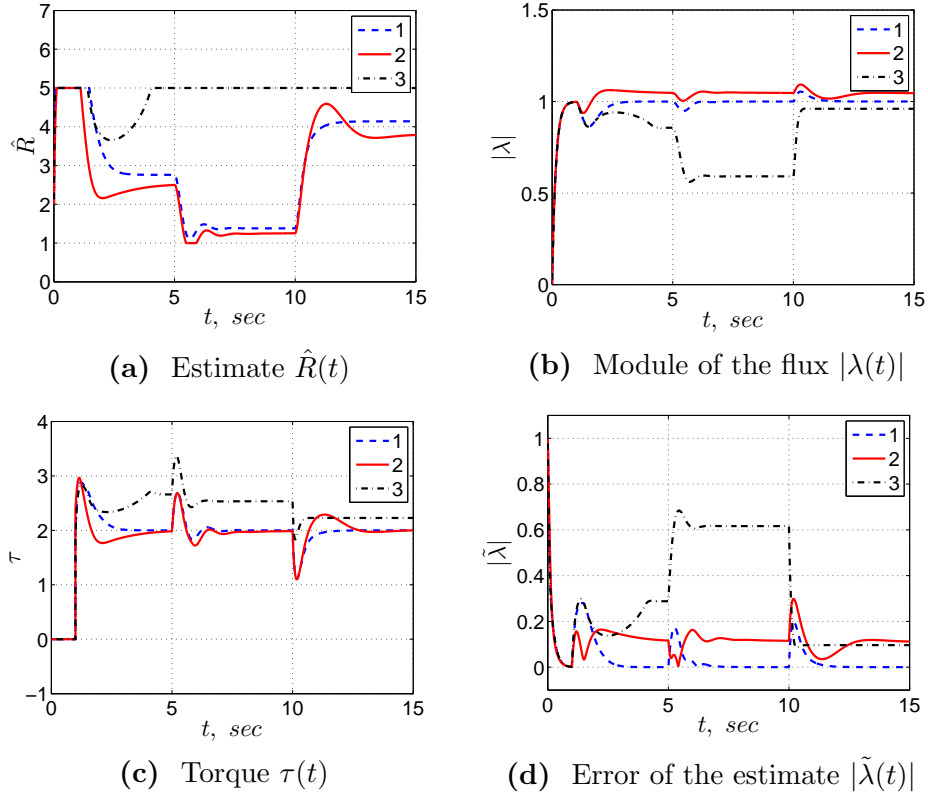
Figure 5: Simulation results of the adaptive torque regulation IFOC of Proposition 2 with \gamma = 50 , z(0) = 2 , \lambda(0) = (0, 0) , \dot{\lambda}(0) = (0, 1) step changes in R and wrong estimates of D and L . 1. (blue line) \hat{D} = 0.7D , \hat{L} = L ; 2. (red line) \hat{D} = 0.9D , \hat{L} = 1.2L ; 3. (black line) \hat{D} = 1.2D , \hat{L} = 0.95L .
