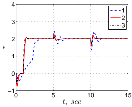
(c) Torque \tau(t)
