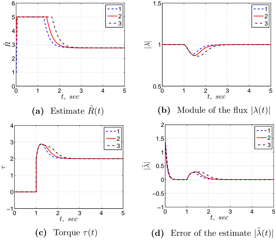
Figure 2: Simulation results of the adaptive torque regulation IFOC of Proposition 2 with \gamma = 100 , \lambda(0) = (1, 0) , \dot{\lambda}(0) = (0, 1) and different initial conditions for z . 1. (blue line) z(0) = 0 ; 2. (red line) z(0) = 3 ; 3. (black line) z(0) = 5 .
