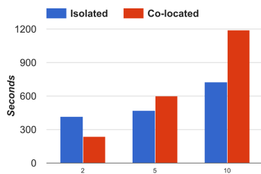
Fig. 1. The deployment-time overhead of the agents; LXD vs co-located.
