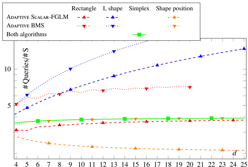
Figure 1: Number of table queries (2D): ADAPTIVE SCALAR-FGLM & ADAPTIVE BMS
