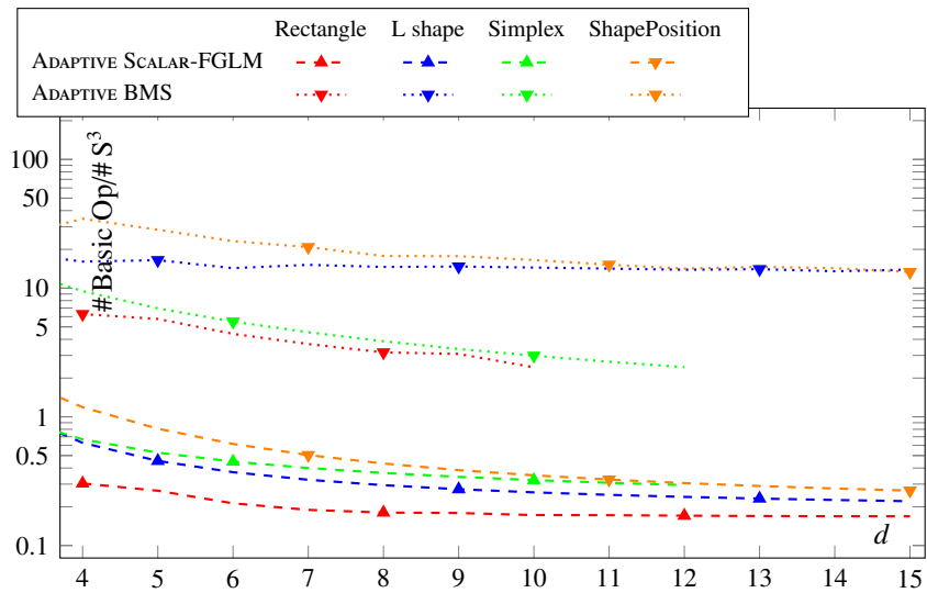
Figure 4: Number of basic operations (3D): ADAPTIVE SCALAR-FGLM & ADAPTIVE BMS
