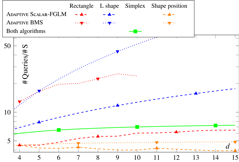
Figure 2: Number of table queries (3D): ADAPTIVE SCALAR-FGLM & ADAPTIVE BMS
