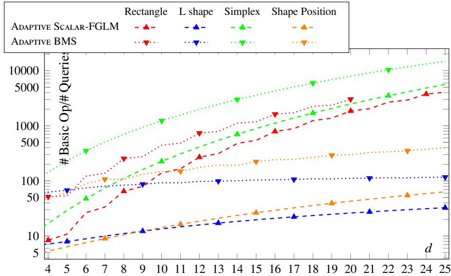
Figure 5: Number of basic operations by queries (2D): ADAPTIVE SCALAR-FGLM & ADAPTIVE BMS
