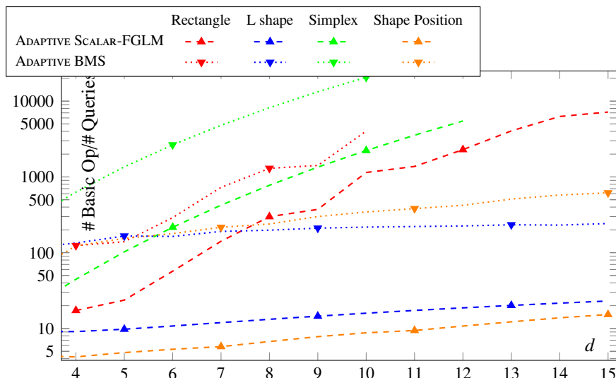
Figure 6: Number of basic operations by queries (3D): ADAPTIVE SCALAR-FGLM & ADAPTIVE BMS
