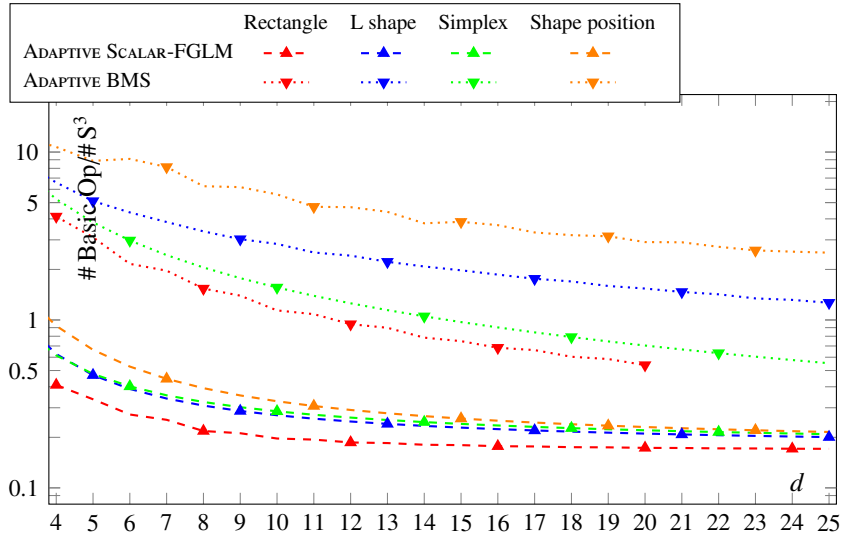
Figure 3: Number of basic operations (2D): ADAPTIVE SCALAR-FGLM & ADAPTIVE BMS
