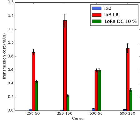
Figure 8: Average transmission cost per bike
