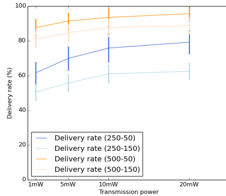
Figure 4: Average delivery rate
