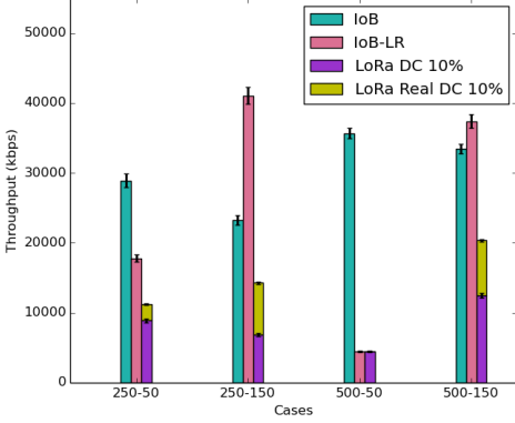
Figure 10: Average throughput
