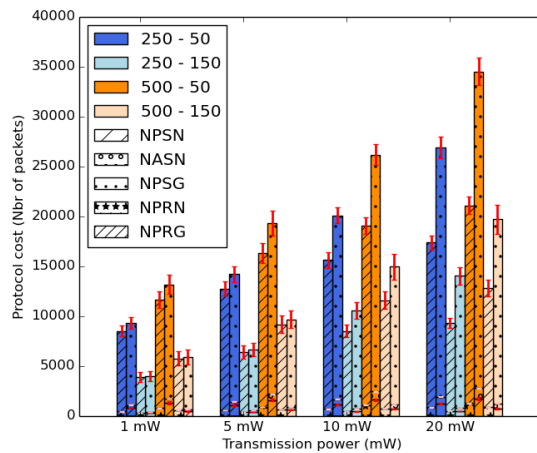
Figure 7: Average protocol cost of IoB
