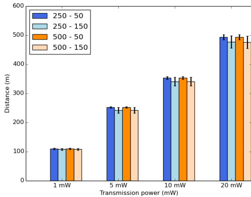
Figure 3: Average distances
