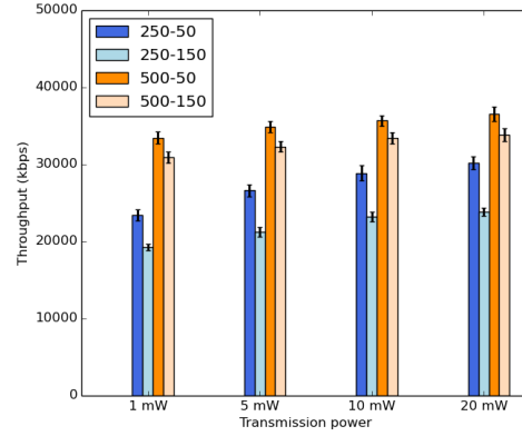
Figure 6: Average throughput
