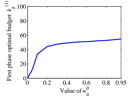
Figure 1: Illustration of the effect of w_{ii}^0 (NetHEPT) with k_g = 100
