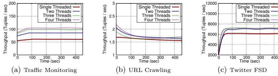
Fig. 5. Parallel Compression Results.
