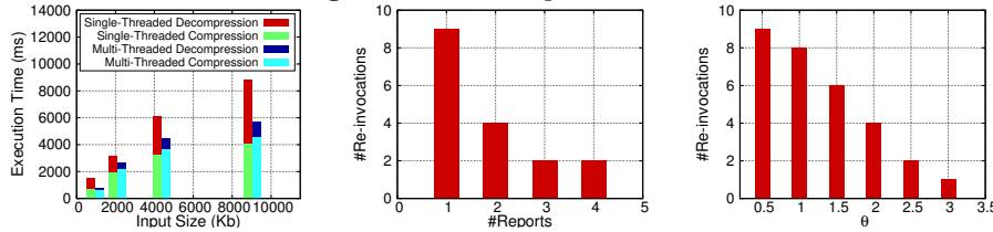
Fig. 6. Impact of data size on compression/decompression time.
