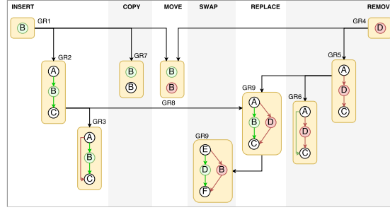
Fig. 5. Example set of graph rules to detect low- and high-level changes
