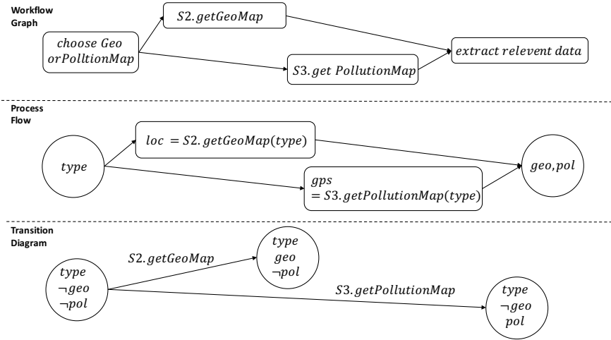
Fig. 10. Process Graph to ASP
