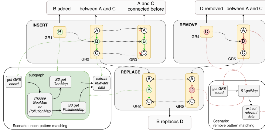
Fig. 9. GR-based change patterns Insert , Remove and Replace
