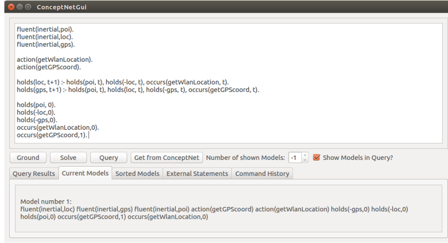
Fig. 11. ASP Viewer [14]
