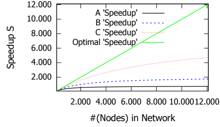
Fig. 4. Speedup S
