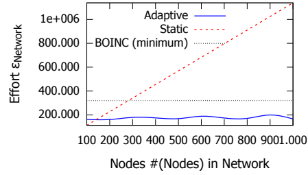
Fig. 6. Cheat Detection Effort – Static vs Adaptive Cheat Detection vs BOINC
