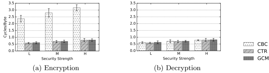
Fig. 2: Performance of AES (cycles per byte)
