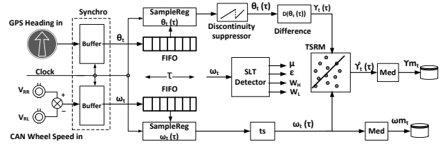
Figure 3: Block Diagram of TedriS training phase. Each consecutive \tau data block of GPS heading ( \theta_t ) and CAN yaw rate ( \omega_t ) are processed by the TSRM to generate the tuple ( \text{Med}(\omega_t), \text{Med}(\hat{\gamma}_t) ) database. Straight Line Trajectory (SLT) provides parameters related to the difference in wheels speeds data.
