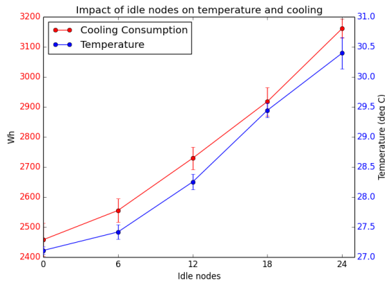
Figure 6: Central cooling consumption and average temperature in the hot aisle (SCS disabled)
