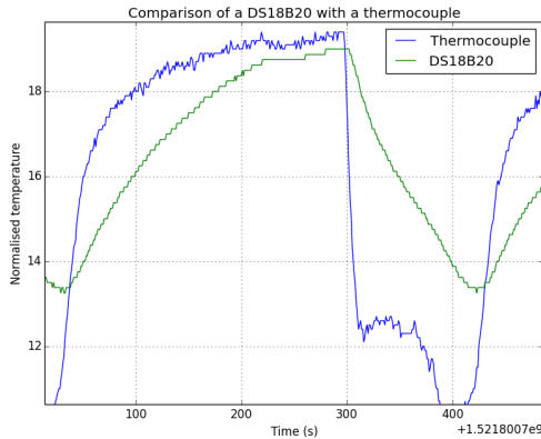
Figure 7: Comparison between DS18B20 and thermocouples
