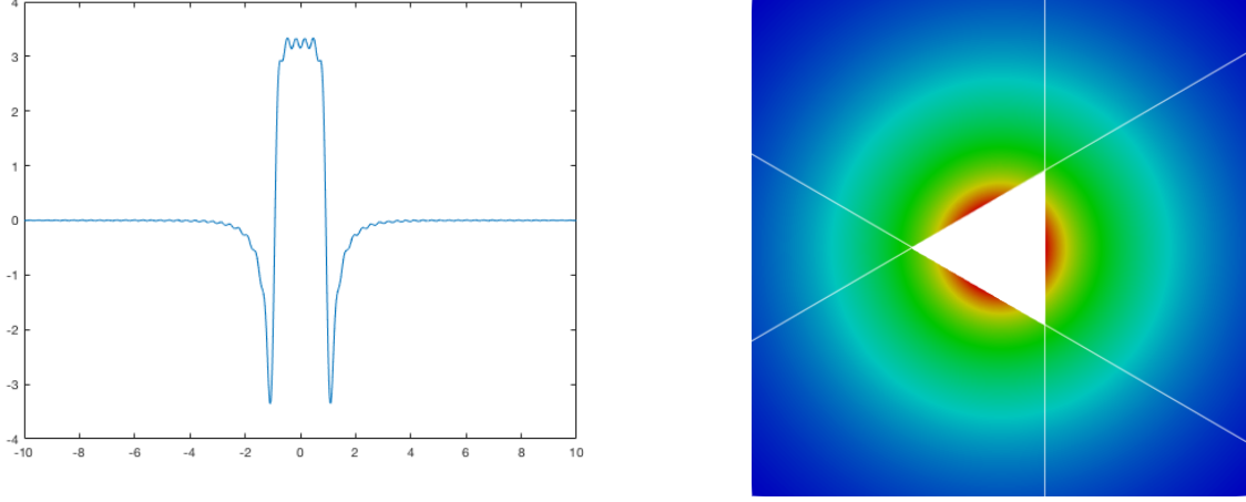
Figure 5: On the left: real part of the Fourier transform \hat{\varphi}_{T,h}^0 . On the right: reconstruction of the solution in \Omega .
