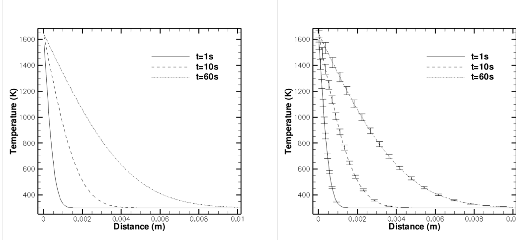
Figure 3: Analytical solution for unidimensional transient heat transfer with fixed surface temperature, for a semi-infinite medium of thermal diffusivity 10^{-7} m 2 /s. Initial temperature of the body: 300 K; surface temperature: 1646 K. Left: temperature profiles for 1, 10, and 60 seconds. Right: error bars in terms of standard deviation when considering two uncertainties.
