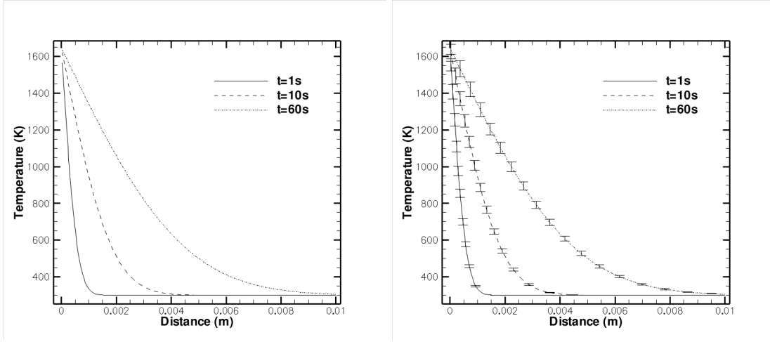
Figure 3: Analytical solution for unidimensional transient heat transfer with fixed surface temperature, for a semi-infinite medium of thermal diffusivity 10^{-7} \text{ m}^2/\text{s} . Initial temperature of the body: 300 K; surface temperature : 1646 K. Left: temperature profiles for 1, 10, and 60 seconds. Right: error bars in terms of standard deviation when considering two uncertainties.
