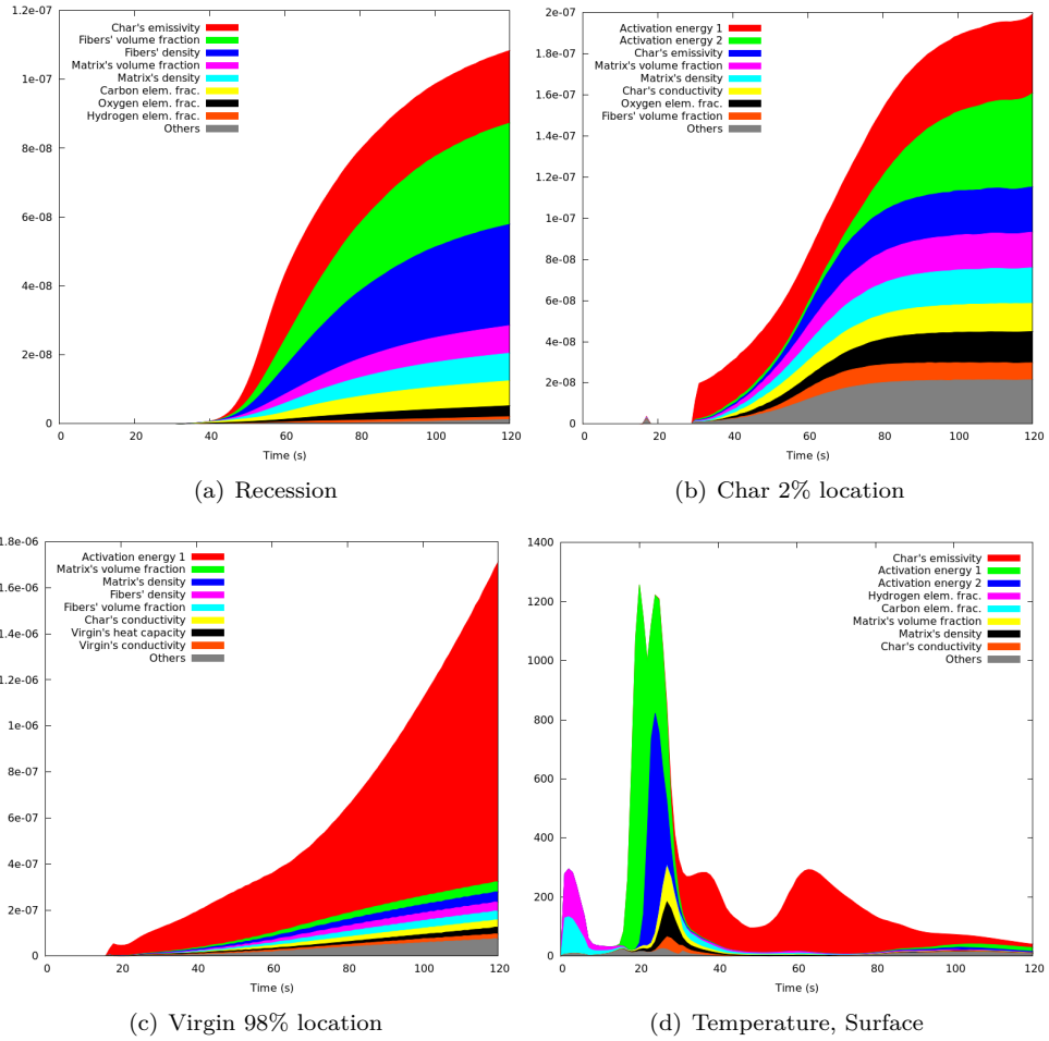
Figure 6: Contributions of each uncertainty to the variance times the variance, computed for several quantities, as a function of time. Units of measure : a) [m^2] vs [s] , b) [m^2] vs [s] , c) [m^2] vs [s] , d) [K^2] vs [s] .
