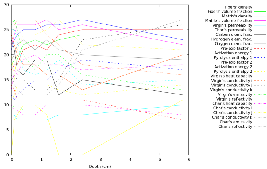
Figure 9: Hierarchy of the uncertain parameters (sorted: the higher, the bigger Sobol index) as a function of depth at t=80 s.
