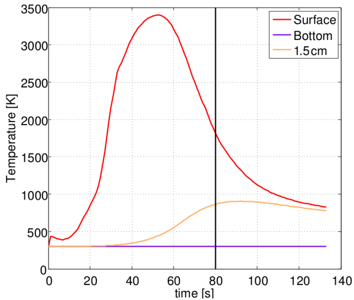
Figure 2: Surface and in-depth temperature obtained with nominal material and pyrolysis gas composition parameters.
