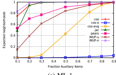
(a) ML-1
