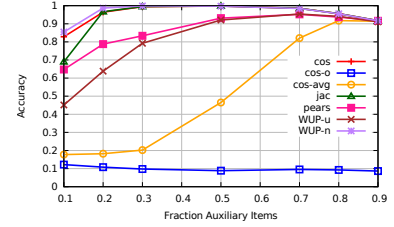
(a) ML-1
