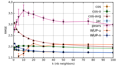
(b) MovieTweetings
