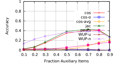
(b) MovieTweetings
