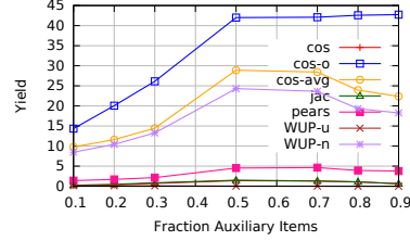
(b) MovieTweetings
