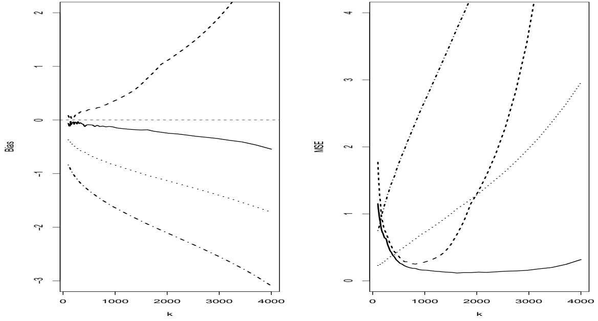
Figure 5: Results on simulated data: Lognormal. Bias (left) and MSE (right) associated with \tilde{Q}_n^{[1]}(\beta_n) (solid line), \tilde{Q}_n^{[2]}(\beta_n) (dotted line), \tilde{Q}_n^{[3]}(\beta_n) (dash-dotted line) and \tilde{Q}_n^{[4]}(\beta_n) (dashed line) as functions of k_n for \beta_n = n^{-2} and n = 5000 .
