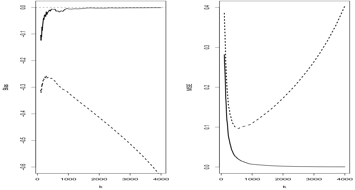
Figure 16: Results on simulated data: super heavy-tail. Bias (left) and MSE (right) associated with \hat{\theta}_n^{(M)} (solid line) and \hat{\theta}_{k_n,n}^{[4]} (dashed line) as functions of k_n for n = 5000 .
