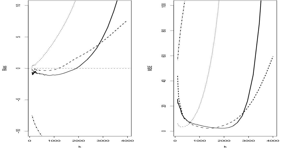
Figure 7: Results on simulated data: Pareto-like. Bias (left) and MSE (right) associated with \tilde{Q}_n^{[1]}(\beta_n) (solid line), \tilde{Q}_n^{[2]}(\beta_n) (dotted line), \tilde{Q}_n^{[3]}(\beta_n) (dash-dotted line) and \tilde{Q}_n^{[4]}(\beta_n) (dashed line) as functions of k_n for \beta_n = n^{-2} and n = 5000 .
