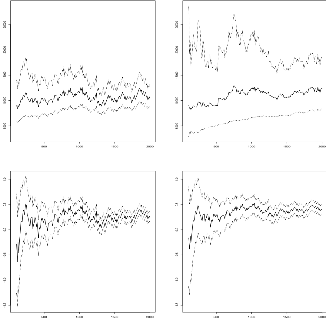
Figure 18: Results on Rhône data. Estimates \tilde{Q}_n^{[1]}(\beta_n) (top left) and \tilde{Q}_n^{[4]}(\beta_n) (top right) of Q(\beta_n) with (\beta_n = 5.5 \cdot 10^{-6}) and their corresponding index estimates \hat{\theta}_n^{(M)} (bottom left) and \hat{\theta}_{k_n, n}^{[4]} (bottom right) as functions of k \in \{100, \dots, 2000\} . The 95% asymptotic confidence intervals are depicted by dotted lines.
