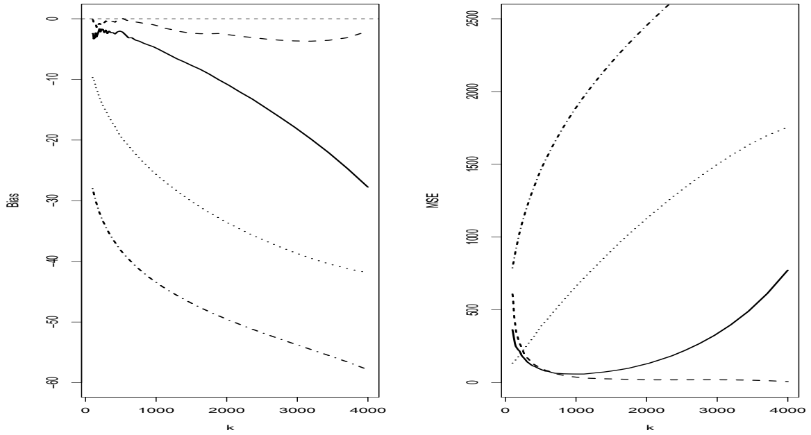
Figure 6: Results on simulated data: Burr. Bias (left) and MSE (right) associated with \tilde{Q}_n^{[1]}(\beta_n) (solid line), \tilde{Q}_n^{[2]}(\beta_n) (dotted line), \tilde{Q}_n^{[3]}(\beta_n) (dash-dotted line) and \tilde{Q}_n^{[4]}(\beta_n) (dashed line) as functions of k_n for \beta_n = n^{-2} and n = 5000 . Top: Burr, bottom: Pareto-like.
