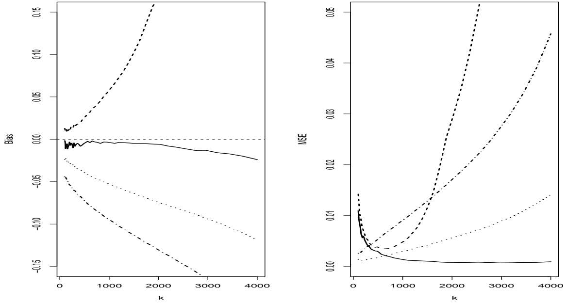
Figure 4: Results on simulated data: Gaussian. Bias (left) and MSE (right) associated with \check{Q}_n^{[1]}(\beta_n) (solid line), \check{Q}_n^{[2]}(\beta_n) (dotted line), \check{Q}_n^{[3]}(\beta_n) (dash-dotted line) and \check{Q}_n^{[4]}(\beta_n) (dashed line) as functions of k_n for \beta_n = n^{-2} and n = 5000 .
