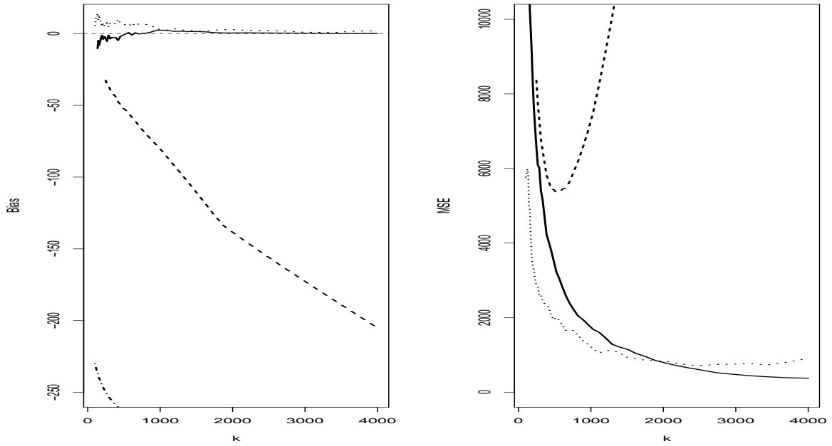
Figure 8: Results on simulated data: super heavy-tail. Bias (left) and MSE (right) associated with \tilde{Q}_n^{[1]}(\beta_n) (solid line), \tilde{Q}_n^{[2]}(\beta_n) (dotted line), \tilde{Q}_n^{[3]}(\beta_n) (dash-dotted line) and \tilde{Q}_n^{[4]}(\beta_n) (dashed line) as functions of k_n for \beta_n = n^{-2} and n = 5000 .
