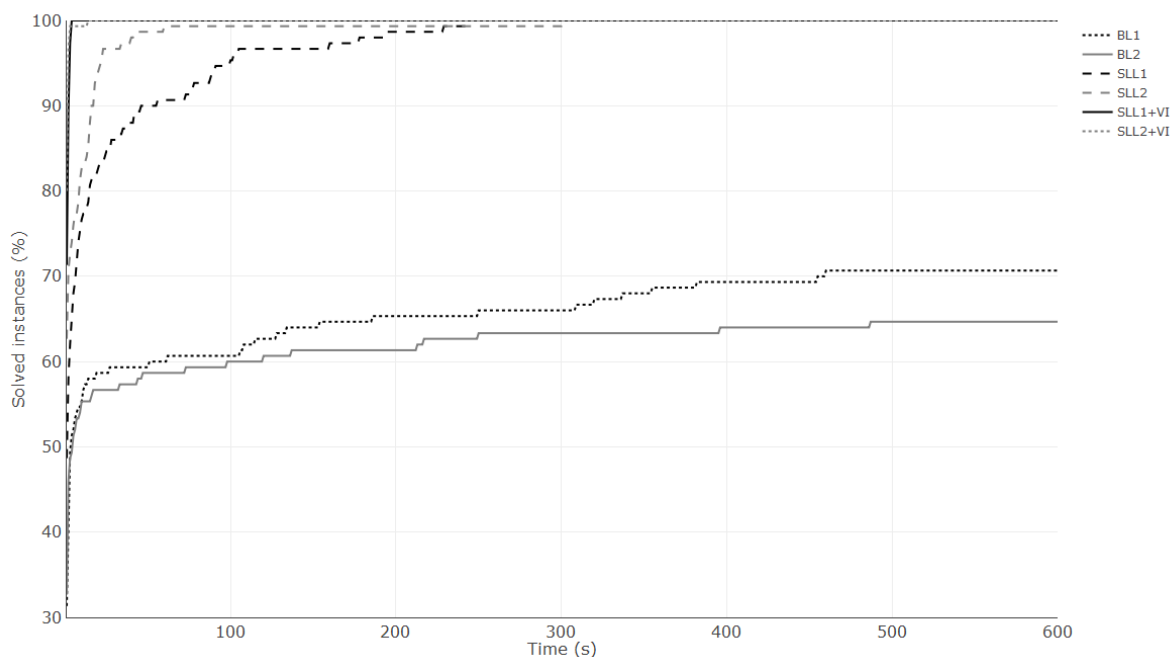
Figure 1: Percentage of instances solved with a time limit by models (BL_1) , (BL_2) , (SLL_1) , (SLL_2) and (SLL_1) , (SLL_2) with the branch-and-cut procedure
