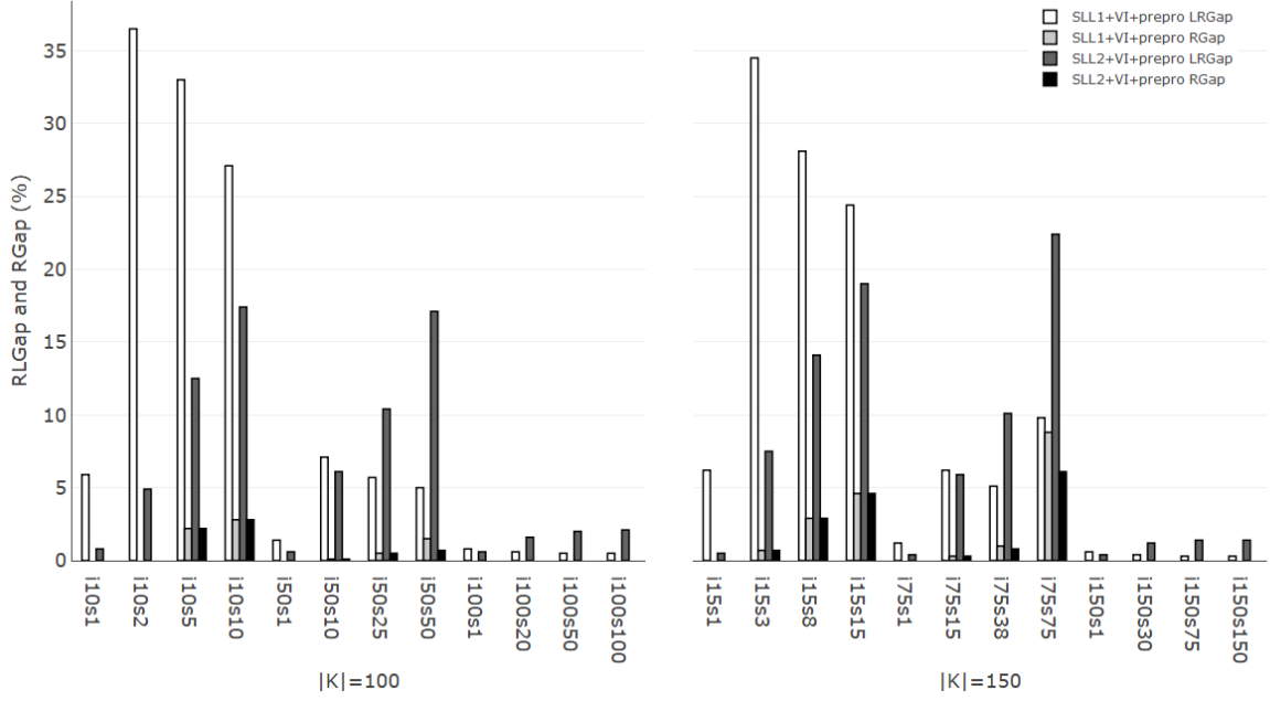
Figure 8: Average duality gaps for models (SLL 1 ) and (SLL 2 ) with the preprocessing techniques. Instances with |K| = 100 are shown in the graphic of the left hand side, and instances with |K| = 150 , in the graphic of the right hand side
