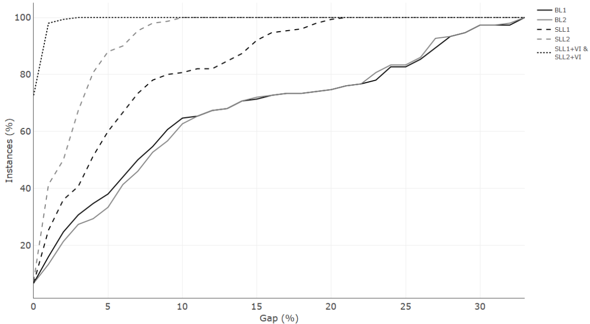
Figure 3: In the ordinate axis it is represented, for models (BL_1) , (BL_2) , (SLL_1) , (SLL_2) and (SLL_1) and (SLL_2) with the branch-and-cut procedure, the percentage of instances with a duality gap less than or equal to that of the axis of abscissas
