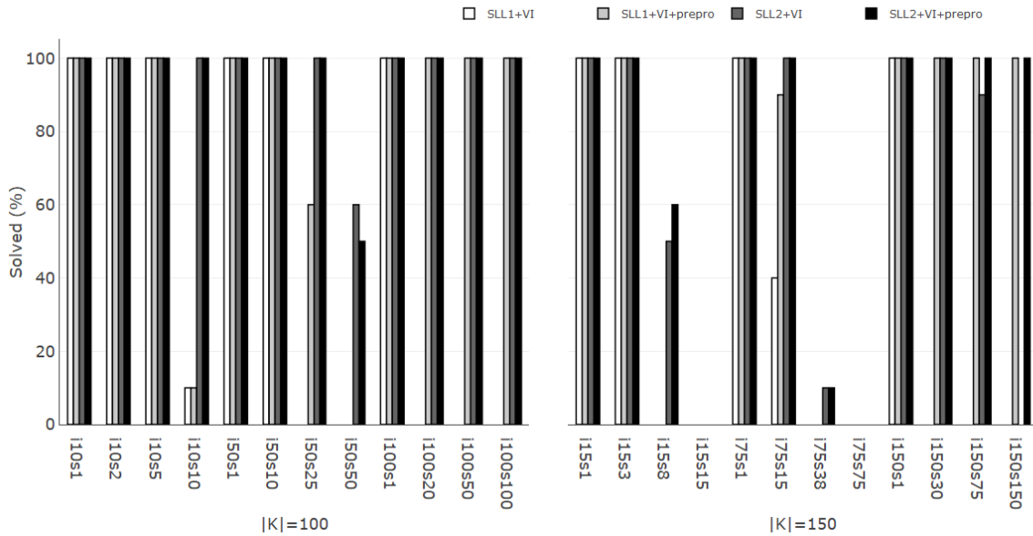
Figure 7: Percentage of solved instances depending on their size. Instances with |K| = 100 are shown in the graphic of the left hand side, and instances with |K| = 150 , in the graphic of the right hand side. The size of the set of products is included after the letter i in the notation of the instances, and the number of products of interest of every customer appears after the letter s
