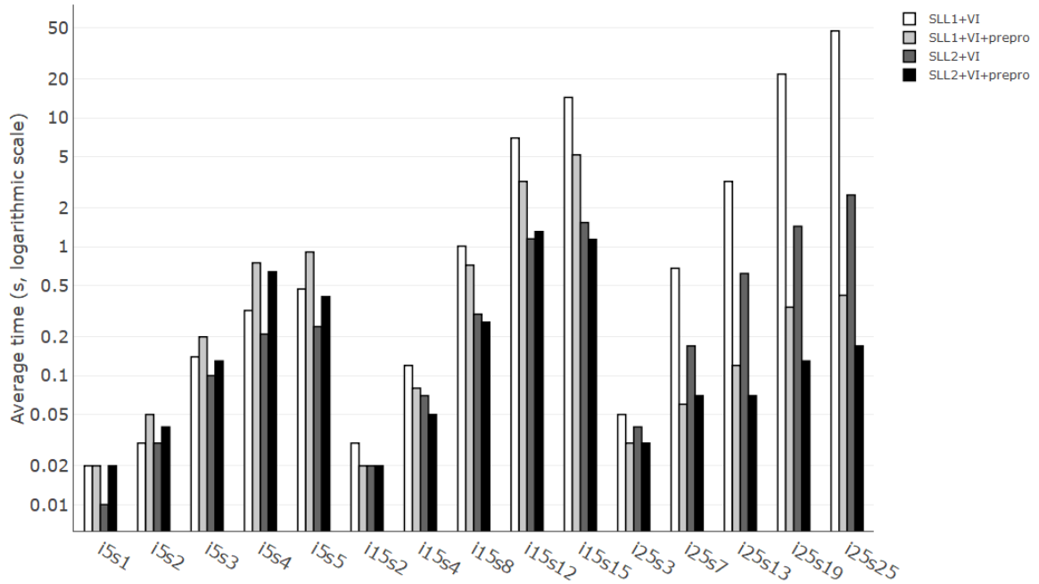
Figure 4: Average time needed to solve instances with |K| = 30 by models (SLL 1 ) and (SLL 2 ), with and without the preprocessing techniques (ten instances averaged per size)
