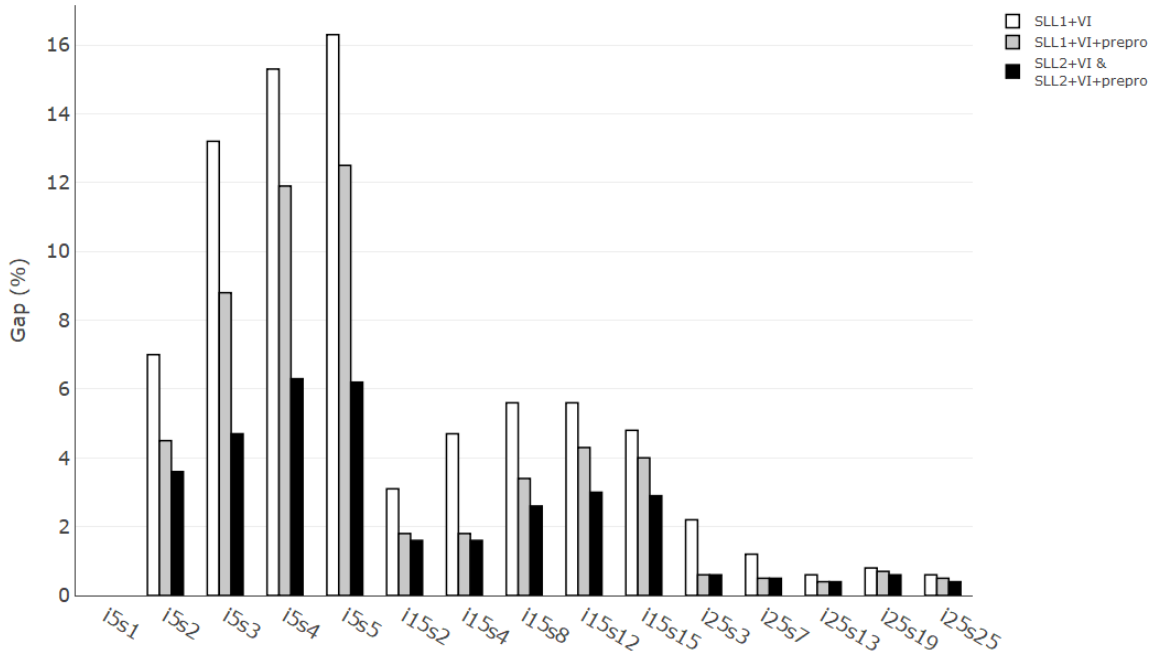
Figure 5: Average duality gaps of the linear relaxation, LRGap, for instances with |K| = 30 by models (SLL 1 ) and (SLL 2 ), with and without the preprocessing techniques (ten instances averaged per size)
