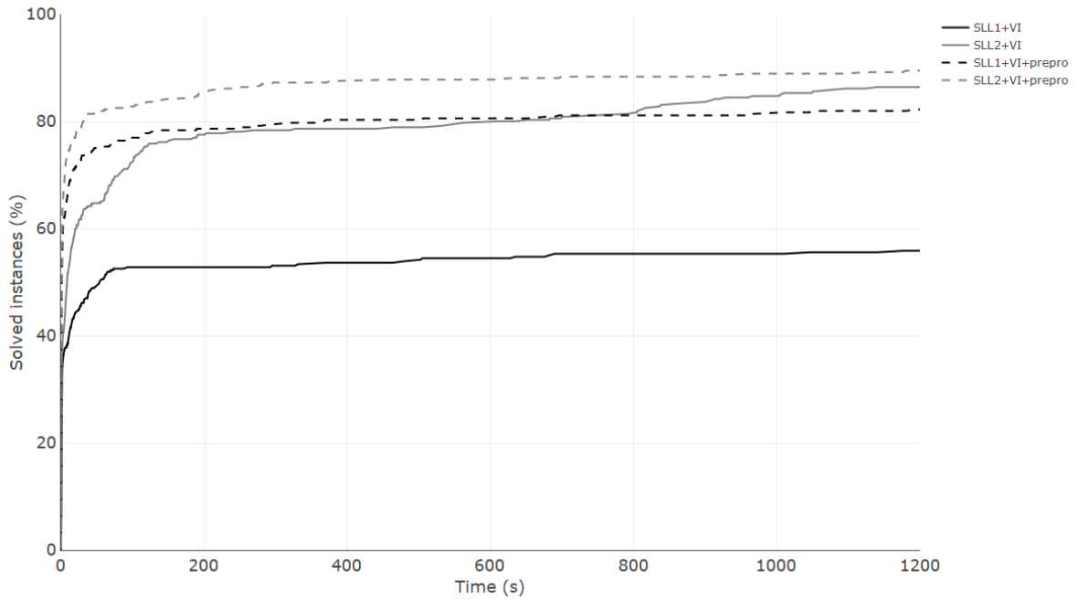
Figure 6: Percentage of instances solved with a time limit by models ( SLL_1 ) and ( SLL_2 ), with and without the preprocessing techniques detailed in Section 6
