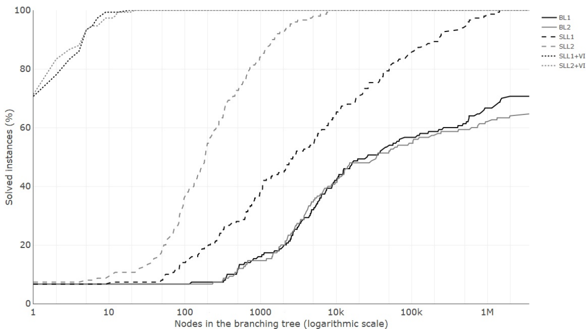
Figure 2: Percentage of solved instances depending on the number of nodes explored in the branching tree by models (BL_1) , (BL_2) , (SLL_1) , (SLL_2) and (SLL_1) , (SLL_2) with the branch-and-cut procedure
