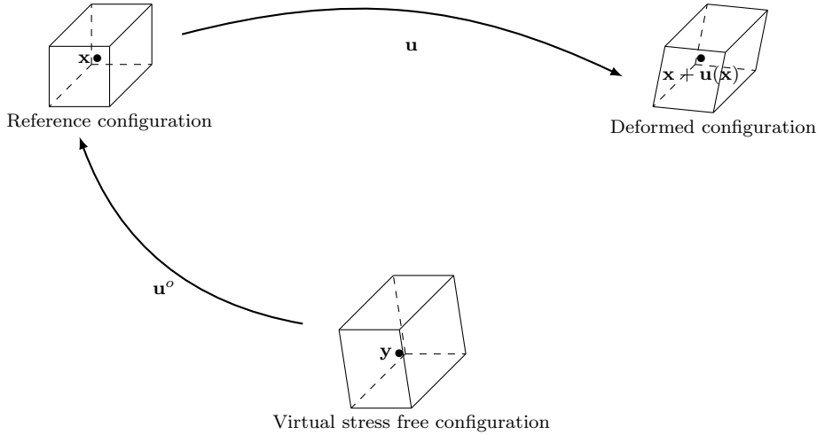
Fig. 2 Representation of an infinitesimal neighborhood of a point \mathbf{x} in the different configurations describing the stored stress, following the presentation in [13]. The reference configuration represents the medium at rest, which means without displacement but possibly with accumulated stress. When released from the stress exerted from the surrounding medium, the infinitesimal neighborhood relaxes to a (virtual) stress free configuration. The accumulated stress is described by the deformation gradient F^o from the virtual stress free configuration to the reference configuration. The neighborhood of \mathbf{x} is distorted through the displacement field \mathbf{u} . The constitutive equation for the medium with accumulated stress is obtained from the constitutive hyperelastic law of the medium, and the deformation from the stress free configuration to the deformed configuration is FF^o , where F = Id + \nabla \mathbf{u} .
