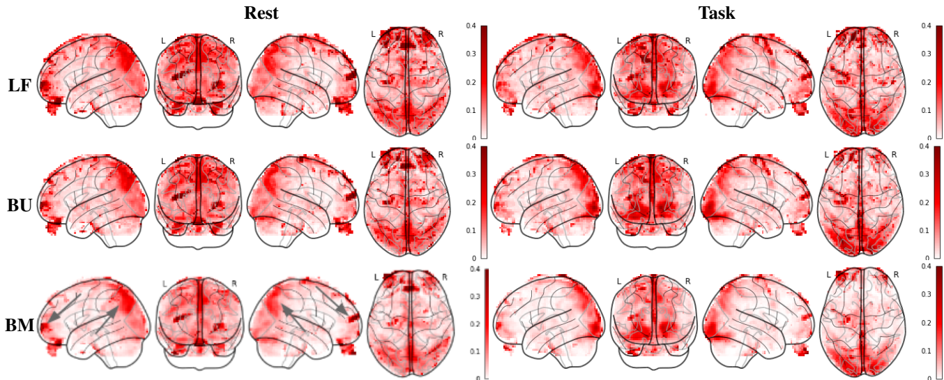
Fig. 1. Group-level estimates of H . From top to bottom \hat{H}_{LF} - 1 , \hat{H}_{BU} - 1 and \hat{H}_{BM} - 1 (1 has been substracted to enhance contrast). From left to right, left-sagittal, coronal, right-sagittal, axial brain slices. These figures have been designed using http://nilearn.github.io . Gray-colored arrows indicate brain regions (PCC, FP) where the multivariate estimate \hat{H}_{BM} gives enhanced contrast.
