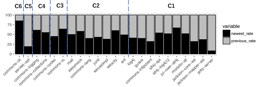
Fig. 5. Figure showing the adoption status rate of each library. The black bar means the adoption rate of newest version. The gray bar means the adoption rate of previous version. As showing by rate, the vertical axis means 100%
