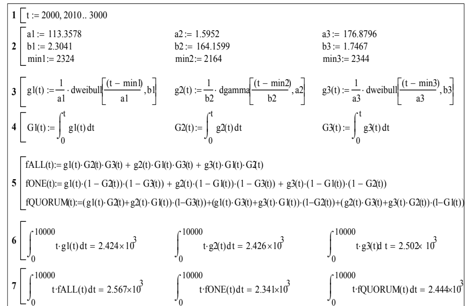
Fig. 7. Mathcad's worksheet.
