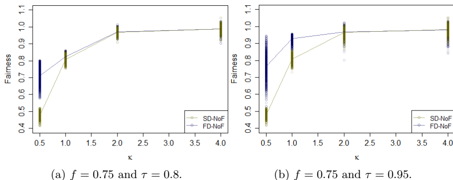
Fig. 1: Average and density of fairness to collaborators along \kappa \in \{0.5, 1, 2, 4\} with SD-NoF and FD-NoF.
