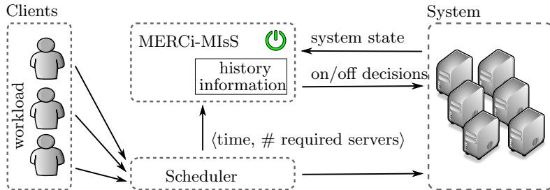
Fig. 2: MERCi-MIS interaction with scheduler and system
