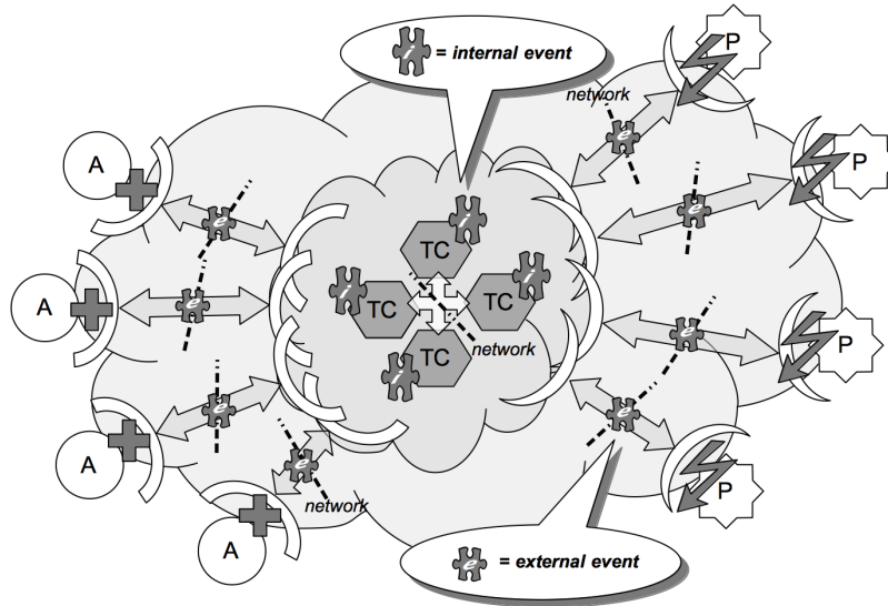
Figure 1. TuCSoN event-based architecture
