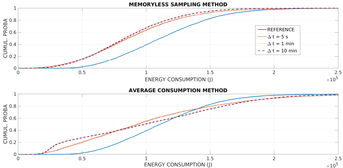
Fig. 5: Consumption distribution for one segment - effect of the Time frame duration
