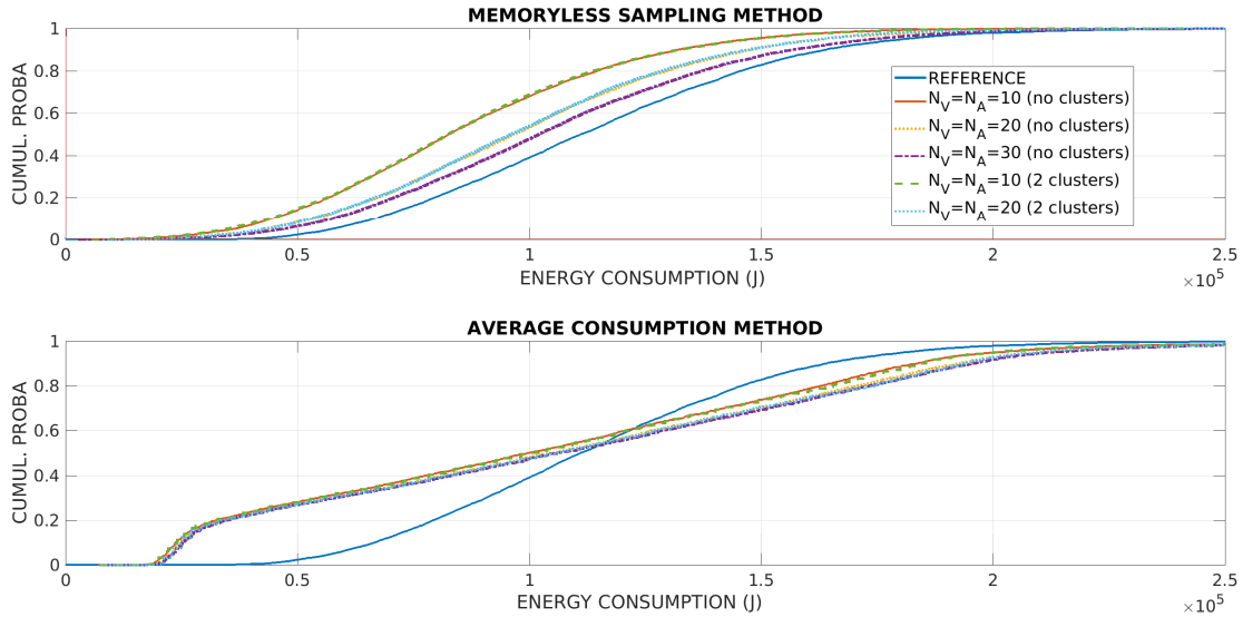
Fig. 4: Consumption distribution for one segment - effect of (v, a) discretization and clustering
