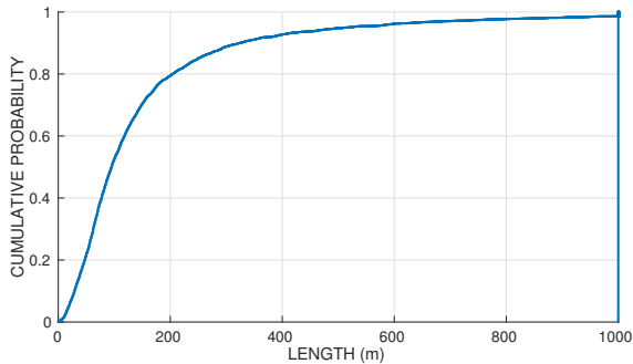
Fig. 1: An illustration of cumulative distribution of the length of road segments.
