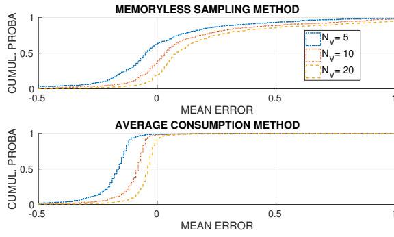
(a) Relative Mean error
