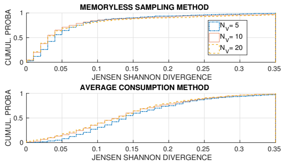
Fig. 7: Speed discretization - Jensen Shannon divergence
