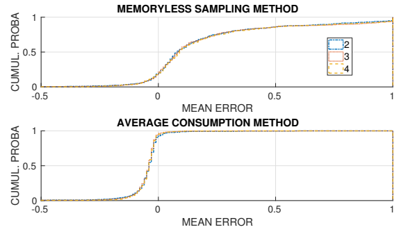
Fig. 11: Number of clusters - Mean error
