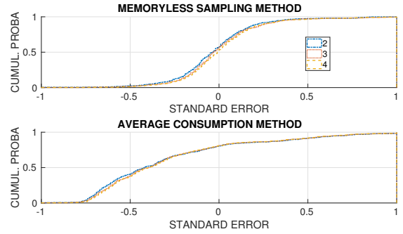
Fig. 12: Number of clusters - Standard deviation error
