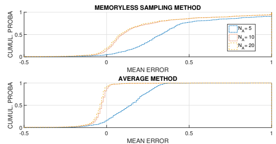
Fig. 8: Acceleration discretization - Mean error
