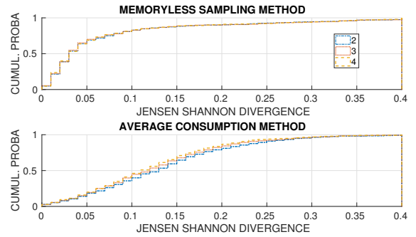
Fig. 13: Numbers of clusters - Jensen Shannon divergence
