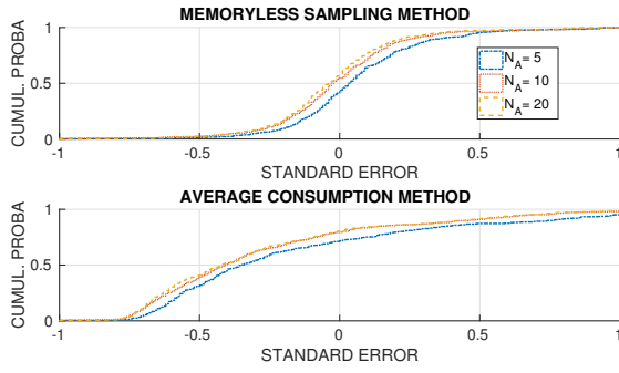
Fig. 9: Acceleration discretization - Standard deviation error
