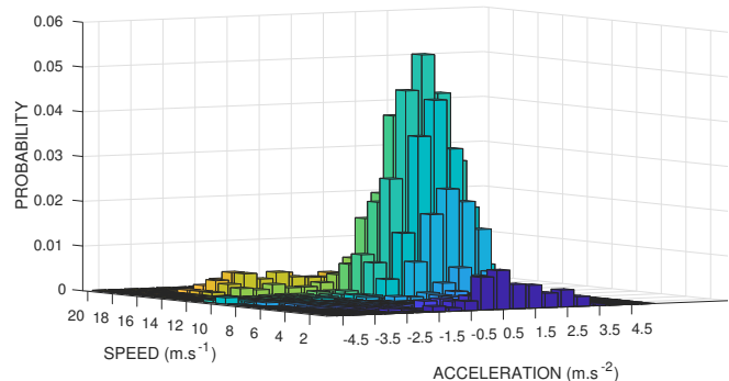
Fig. 2: Example of Speed/Acceleration distribution.
