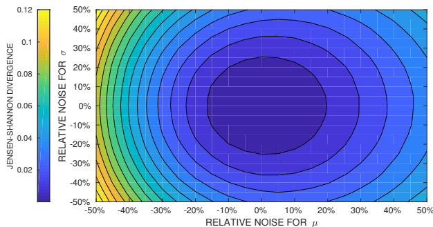
Fig. 3: Jensen Shannon divergence for a noised Gaussian distribution with base parameters \mu = \sigma = 1
