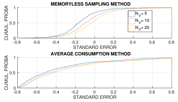
(b) Relative Standard deviation error
