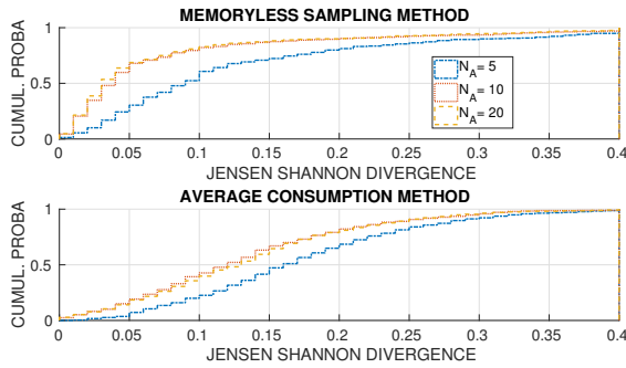
Fig. 10: Acceleration discretization - JS divergence
