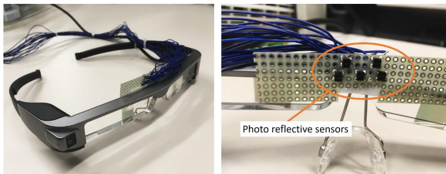
Fig. 3. The appearance of the DecoTouch
