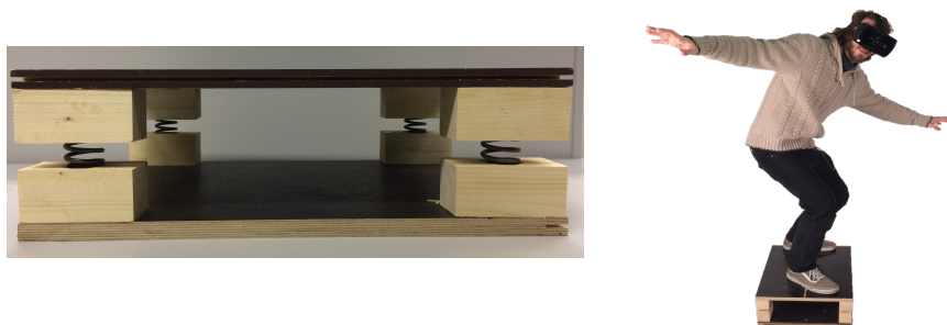
Fig. 3. The updated springboard iteration of the hoverboard device.
