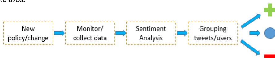
Fig. 9. Sentiment Analysis
