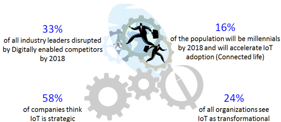
Fig. 1. Digital Transformation [11]
