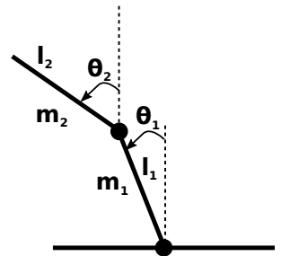
Fig. 2. The pendubot system (with some friction with coefficients b_1, b_2 ). The system has four continuous state variables: two joint angles and two joint angular velocities. The angles of the joints, \theta_1 and \theta_2 , are measured anti-clockwise from the upright position. The pendubot starts hanging down and the goal is to find a policy such that the pendubot swings up and then balances in the upright position. Each episode lasts 2.5 s and the control rate is 20 Hz. We use a distance based reward function as in [8].
