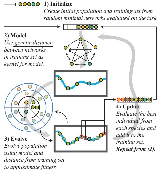
Figure 1: Surrogate-Assisted NEAT Overview
