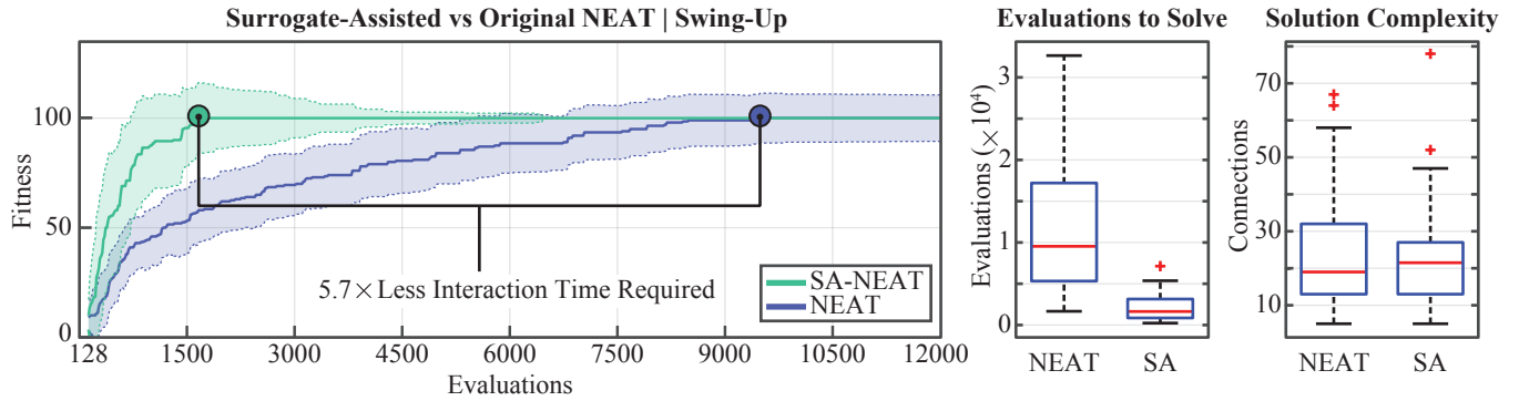
Figure 5: Cart-Pole Swing-Up: Evaluations to Solve Comparison of median best fitness found over 50 trials of SA-NEAT and NEAT on the cart-pole swing-up task. Shaded region indicates one standard deviation from the median. SA-NEAT solved the task in a median of 1664 evaluations, while NEAT required 9488, nearly six times the number of evaluations. Even the most data-efficient quartile of NEAT runs required as many evaluations as the least data-efficient SA-NEAT runs. The complexity of solutions found in each case are similar, demonstrating that the same variable dimensional space explored by NEAT is also explored in the surrogate-assisted variant.
