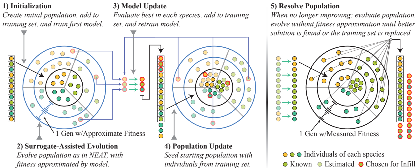
Figure 4: Surrogate-Assisted NEAT
