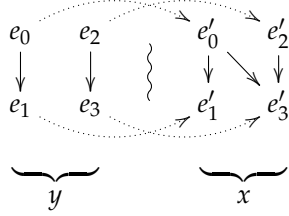
Fig. 2. Two partial strings x and y such that x \sqsubseteq y provided all the labels are preserved, e.g. \alpha_x(e'_0) = \alpha_y(e_0) .
