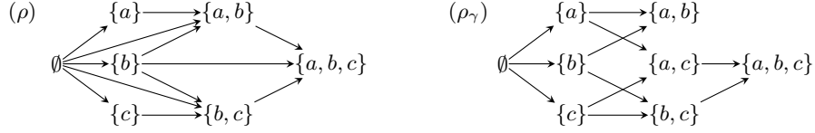
Figure 3. Transition graphs of RCEs with resolvable conflict (\rho) and disabling (\rho_\gamma) .
