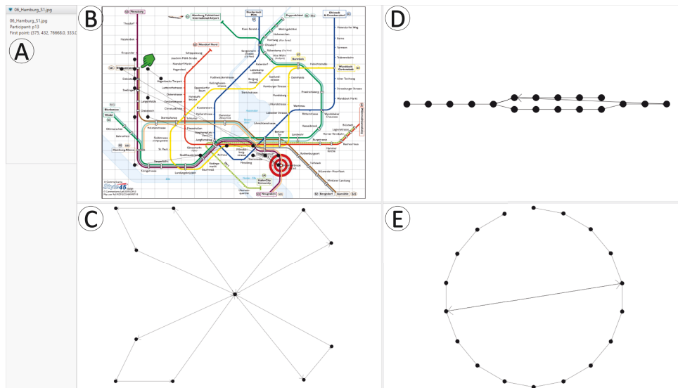
Figure 1. In this example, A) depicts the list of participants and stimuli loaded. B) shows an example stimulus with a 20×20 grid and the generated graph. The same fixation data shown using a C) a force-directed, D) hierarchical, and E) a radial layout.
