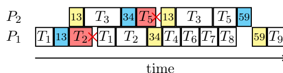
Figure 4: Sample execution of the application in Figure 3 with two failures striking during the execution of T_2 on P_1 and that of T_5 on P_2 , with crossover checkpoints. Label ij indicates the file from T_i to T_j . Now T_4 can start before the re-execution of T_3 since its output was checkpointed.
