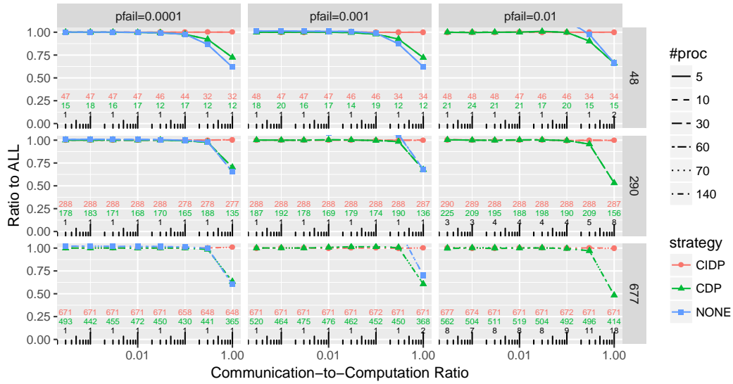
Figure 17: Performance of the different checkpointing strategies for Sipt using HEFTC for task mapping and scheduling.
