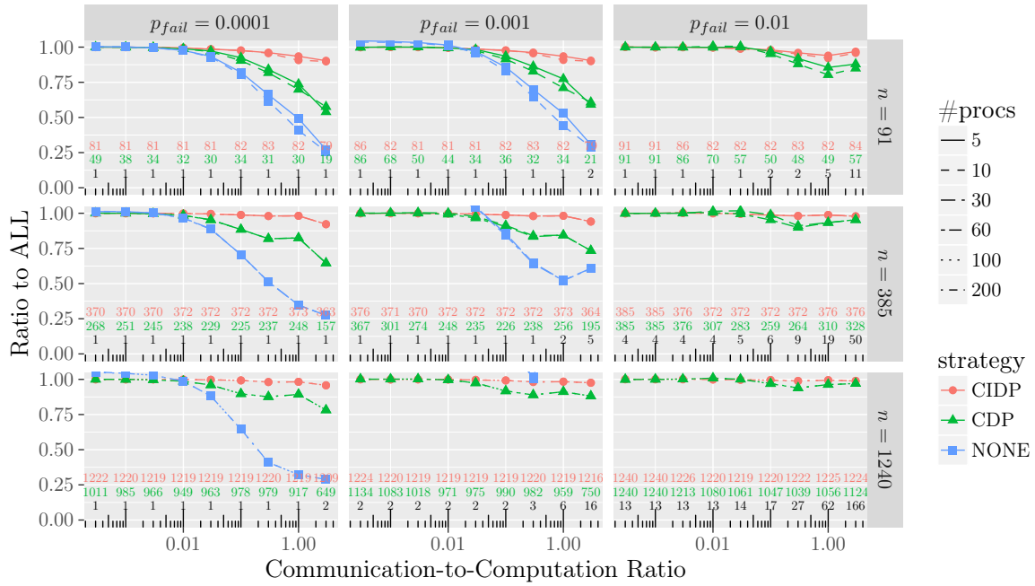
Figure 13: Performance of the different checkpointing strategies for QR using HEFTC for task mapping and scheduling.
