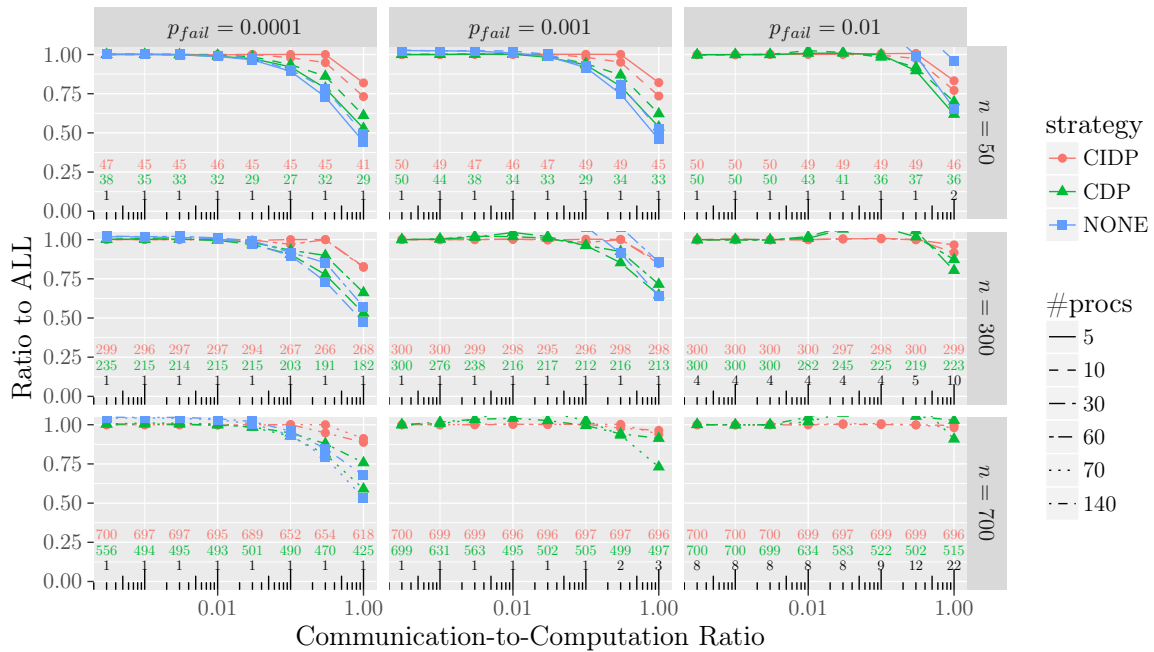
Figure 17: Performance of the different checkpointing strategies for CyberShake using HEFTC for task mapping and scheduling.
