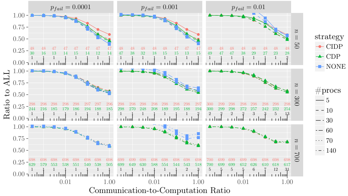
Figure 14: Performance of the different checkpointing strategies for Montage using HEFTC for task mapping and scheduling.
