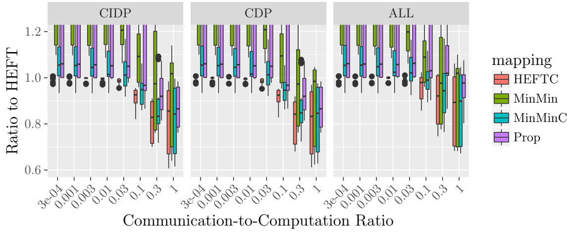
Figure 20: Relative performance of the four task mapping and scheduling strategies and of PROPCkPT for Ligo.
