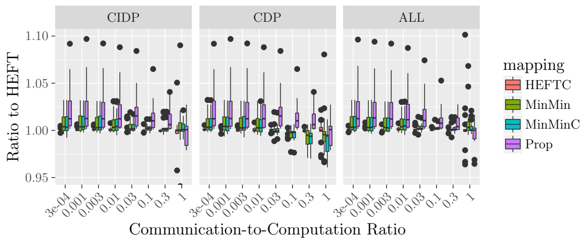
Figure 19: Relative performance of the four task mapping and scheduling strategies and of PROPCKPT for Montage.
