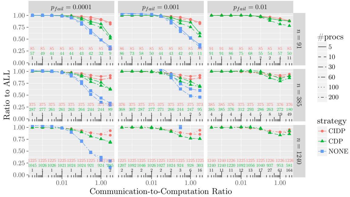
Figure 12: Performance of the different checkpointing strategies for LU using HEFTC for task mapping and scheduling.
