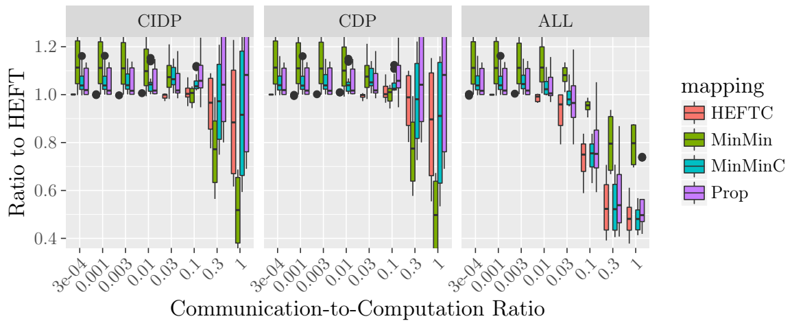
Figure 21: Relative performance of the four task mapping and scheduling strategies and of PROPCkPT for Genome.
