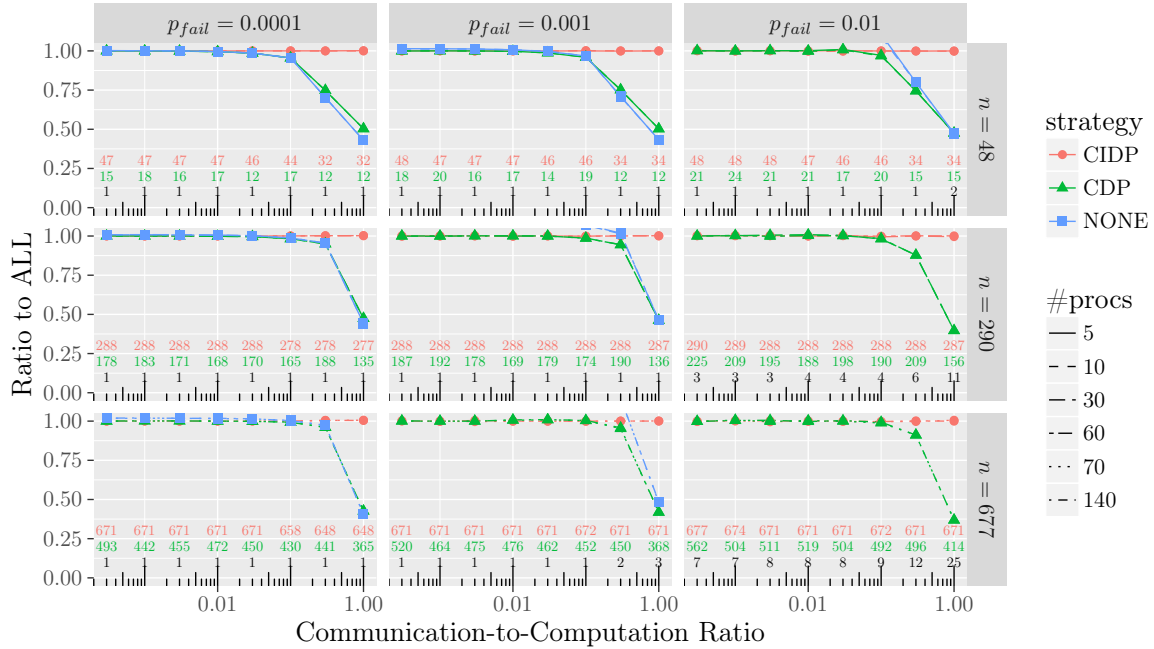
Figure 16: Performance of the different checkpointing strategies for Sipht using HEFTC for task mapping and scheduling.
