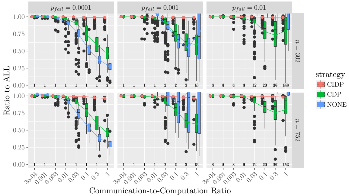
Figure 18: Average performance of the different checkpointing strategies for the STG task graphs using HEFTC for task mapping and scheduling.
