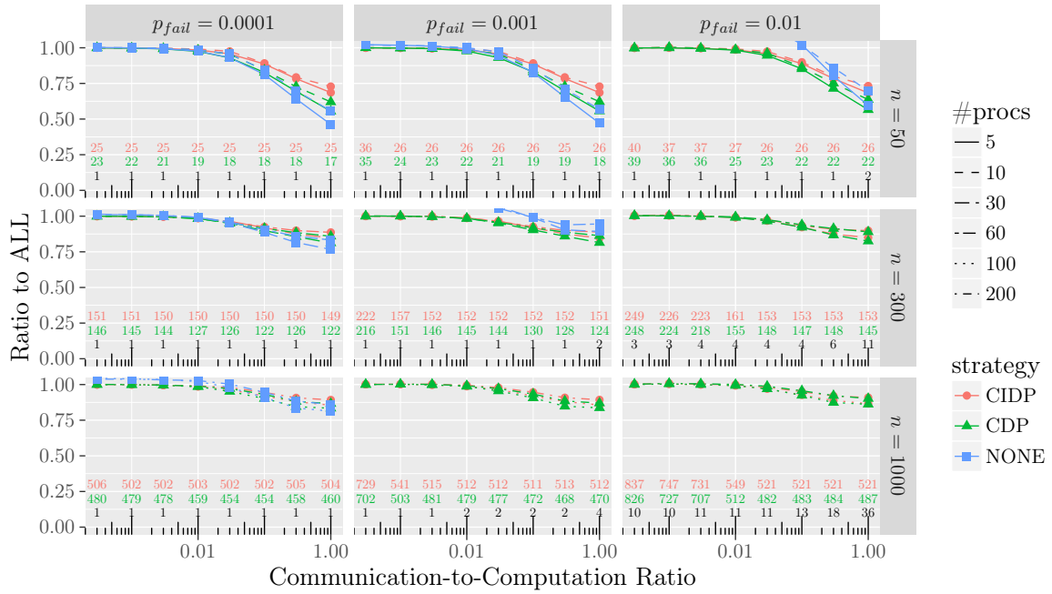
Figure 15: Performance of the different checkpointing strategies for Ligo using HEFTC for task mapping and scheduling.
