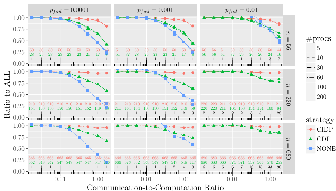
Figure 11: Performance of the different checkpointing strategies for Cholesky using HEFTC for task mapping and scheduling.
