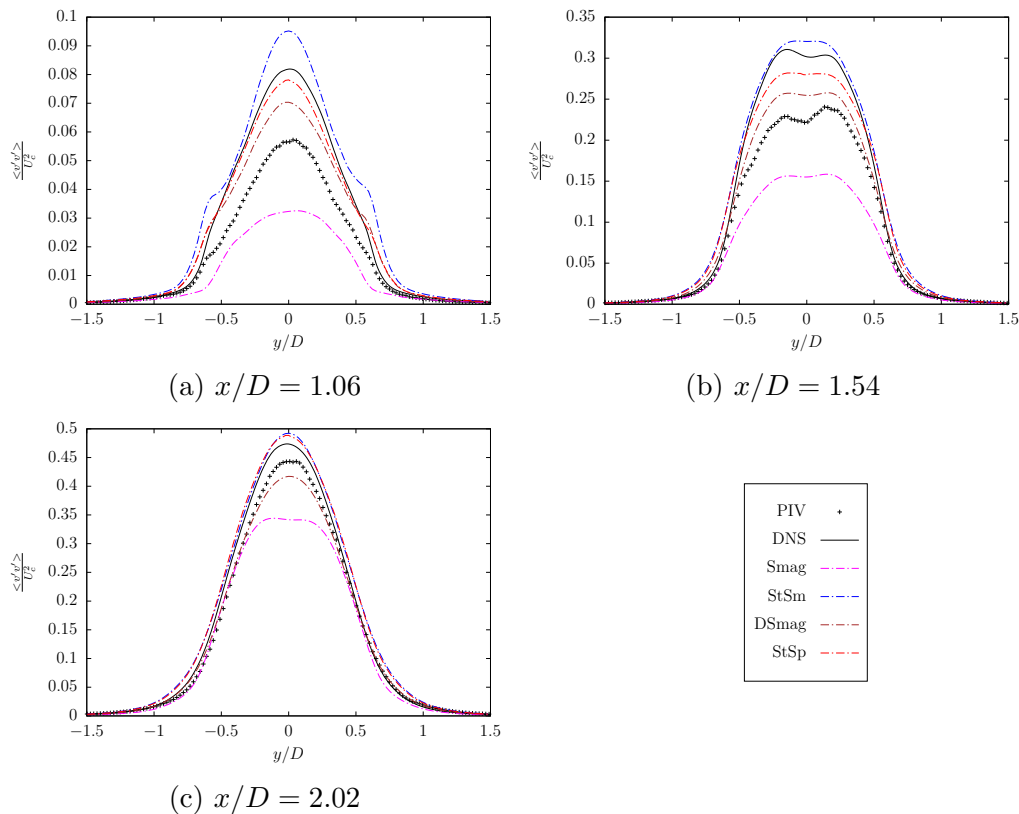
Figure 5: Lateral rms velocity ( v'v' ) fluctuations at 1.06D, 1.54D, and 2.02D in the wake of the circular cylinder.
