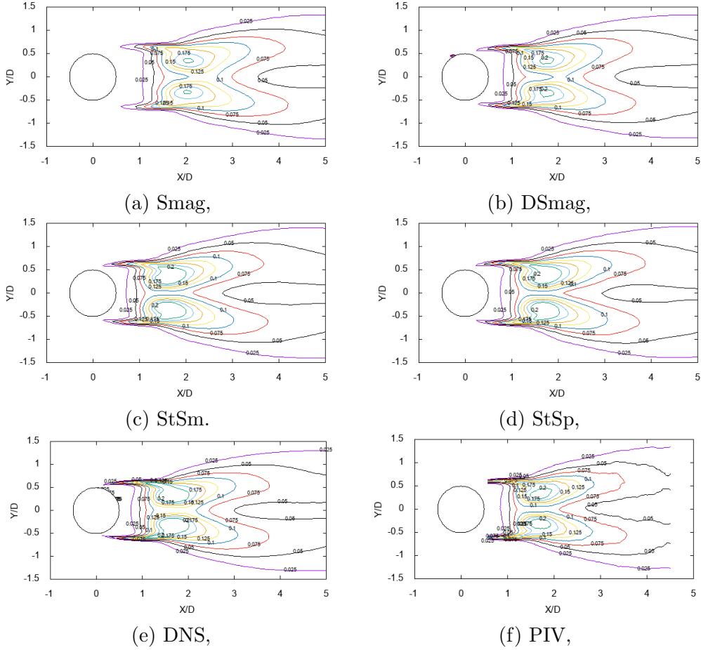
Figure 9: 2D isocontours of time averaged fluctuating streamwise velocity ( u'u' ).
