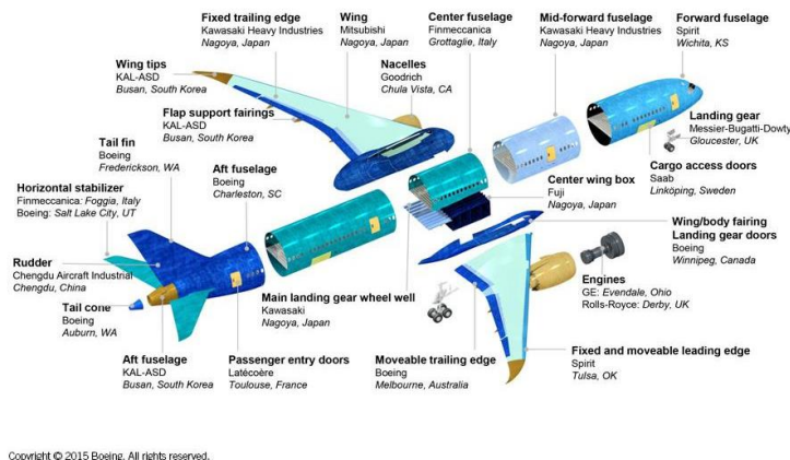
Fig. 6. Boeing 787 Breakdown 1
