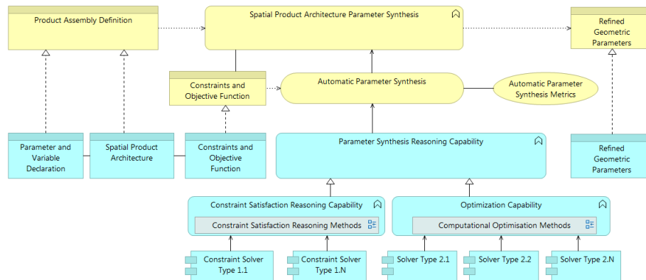
Fig.3. Template for Spatial Product Architecture Parameter Synthesis Task
