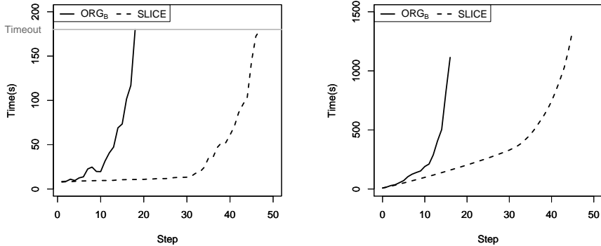
(a) Max verification time for each step (b) Total verification time for each step
