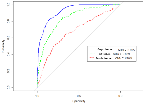
Fig. 5. Performance in term of AUC using different feature without sampling preprocessing.
