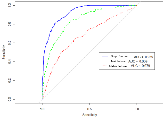
Fig. 5. Performance in term of AUC using different feature without sampling preprocessing.
