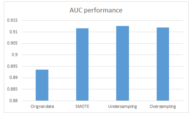
Fig. 6. Performance in term of AUC values using preferential attachment and TF-IDF values.
