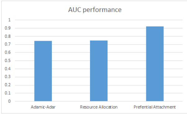
Fig. 4. Performance in term of AUC values using different graph similarity functions.
