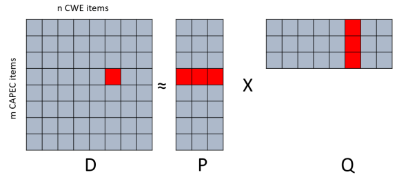
Fig. 1. Matrix factorization
