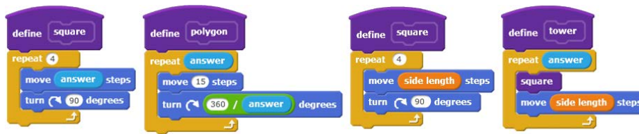
Fig. 4. Definitions generalised by using answer and variables as indirect parameters
