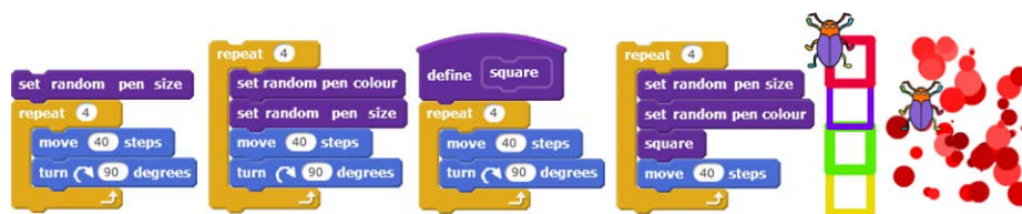
Fig. 3. Defining, using and modifying new blocks in different contexts
