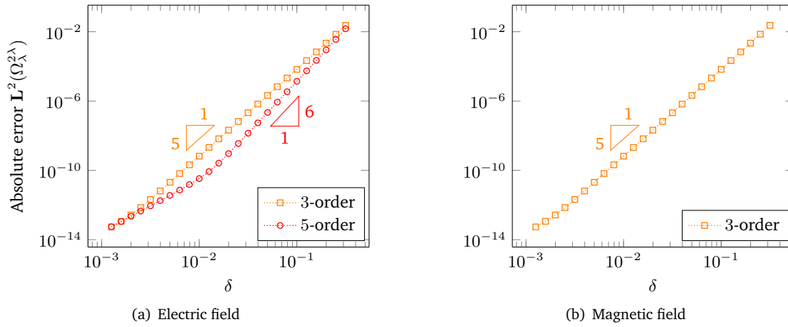
Figure 9: Absolute \mathbf{L}^2 -errors for the far-field approximations associated to Test 2 with \lambda = 5 and w = 5
