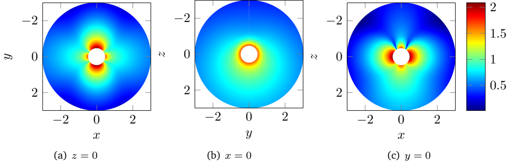
Figure 5: Cross sections of the x -coordinates of the scattered electric field modulus in logarithmic scale associated to Test 2 with \lambda = 5 and w = 5
