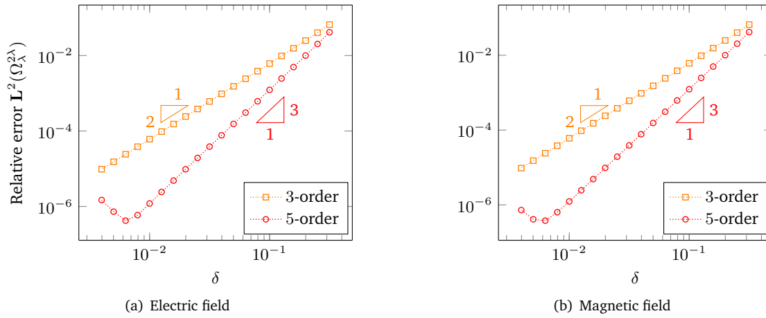
Figure 11: Relative \mathbf{L}^2 -errors for far-field approximations associated to Test 1 with \lambda = 5
